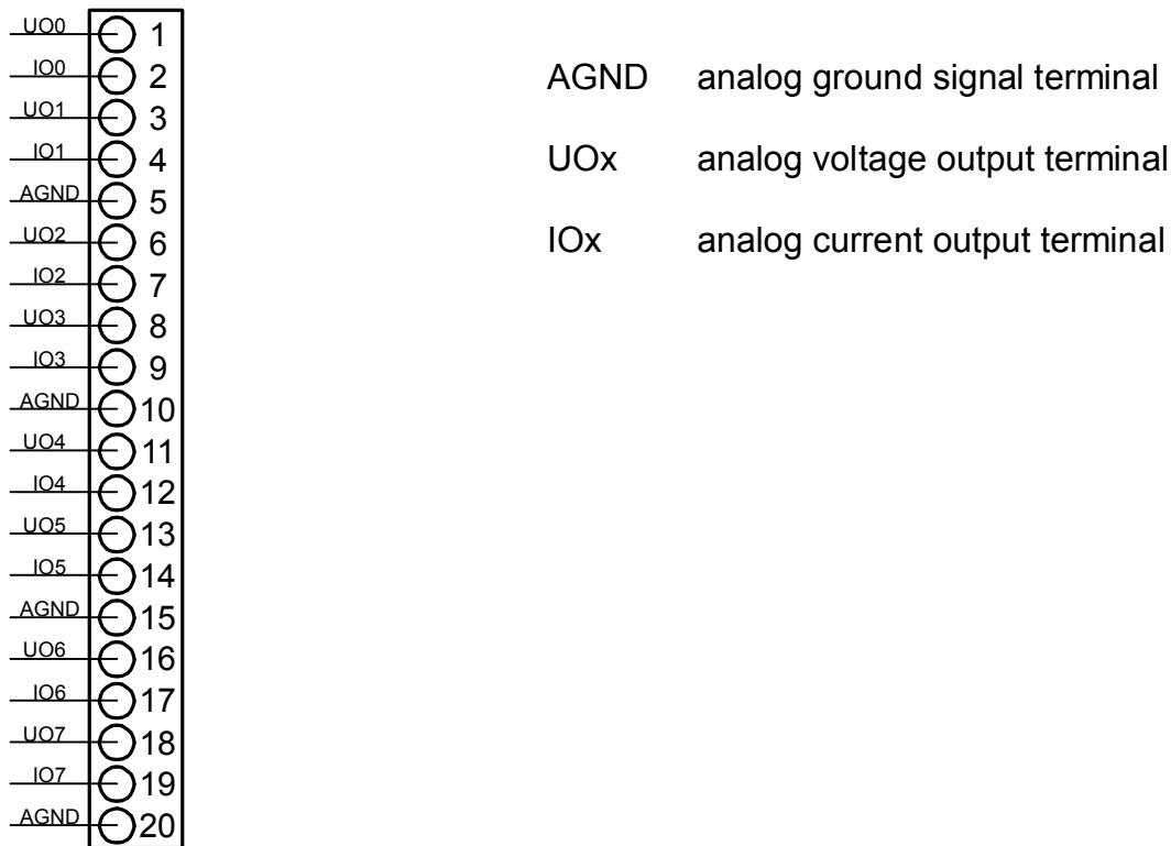
Fig. 5.1: Terminal board connection of the OT-7652 module
