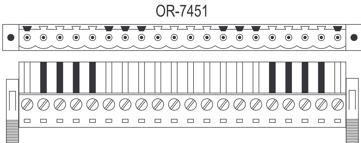
Fig. 9.1: Connector code of the OR-7451 module
