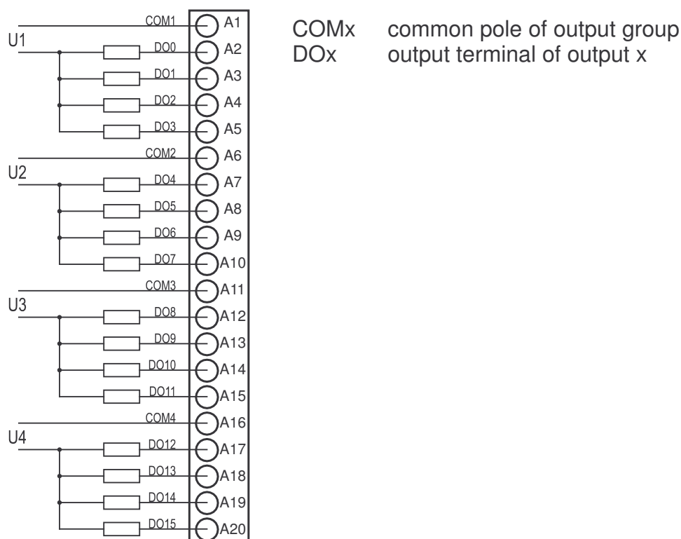
Fig. 5.1: Connector connection of the OR-7451 module
