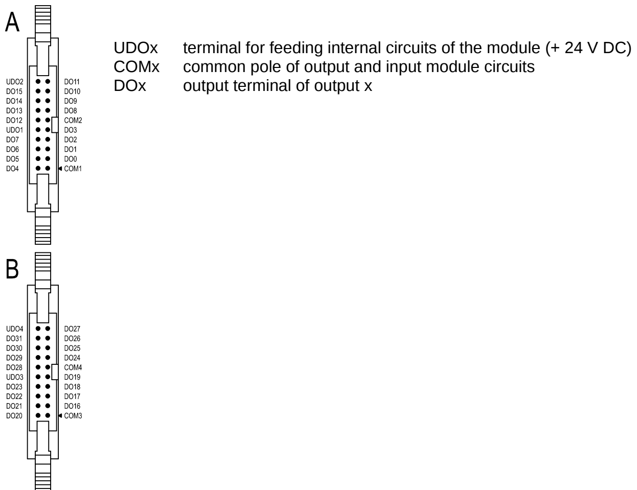
Fig. 5.1: Connector connecting of the OS-7411 module
