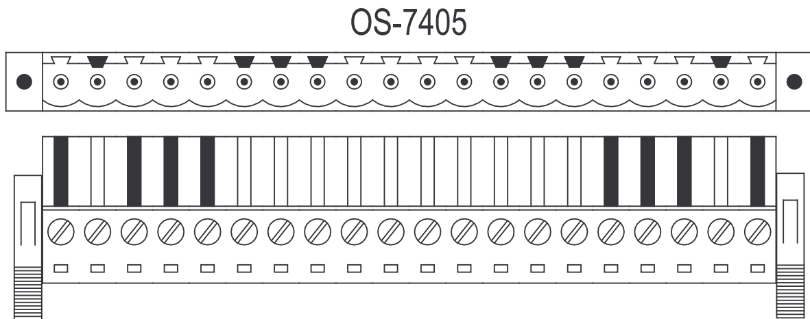
Fig. 9.1 Connector code of the OS-7405 module
