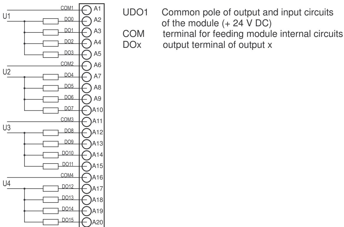
Fig. 5.1: Connector connection of the OS-7405 module
