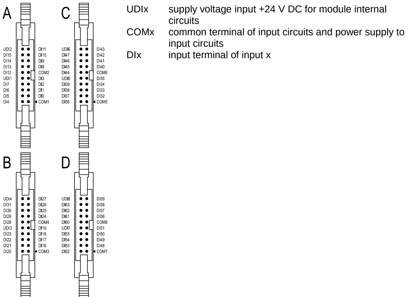
Figure 5.1: Connector connection of the IB-7310 module
