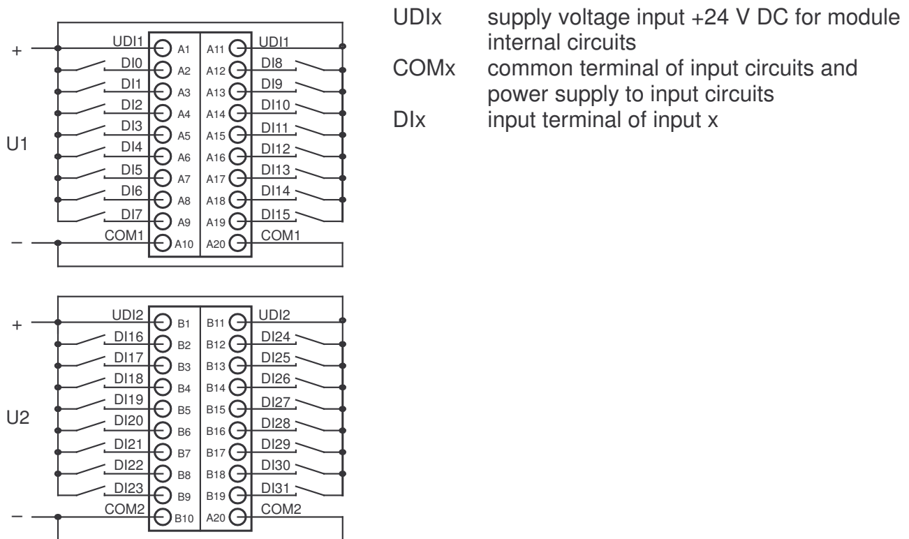
Figure 5.1: Connector connection of the IB-7302 module
