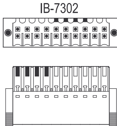
Fig. 9.1: Connector code for module IB-7302
