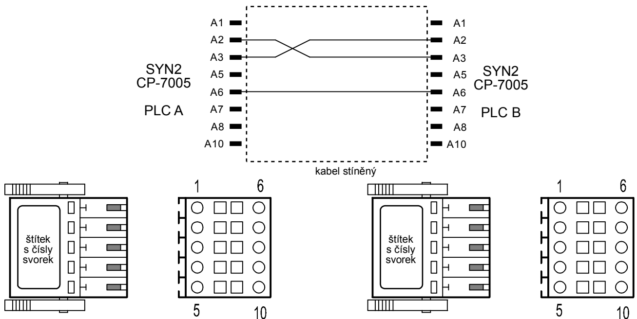
Fig. 5.1 Connection of the CP-7005 SYN2 interfaces (redundant connection)
