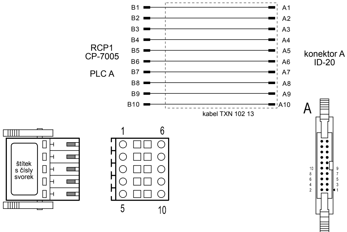
Fig. 5.2 Connection of CP-7005 RCP1 interface (PLC A) and connector A of ID-20 module
