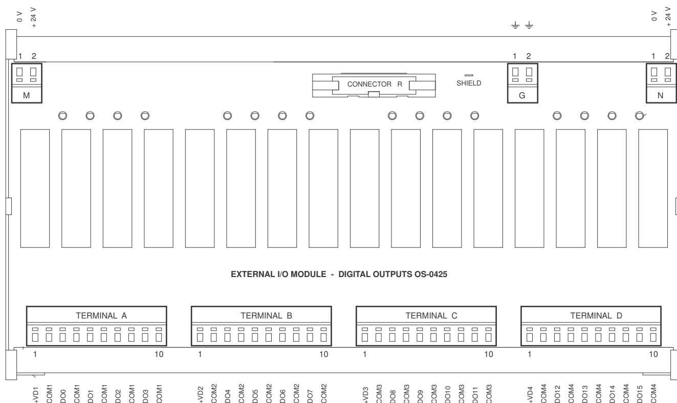
Fig. 5.1: Connector connection of the OS-0425 module
