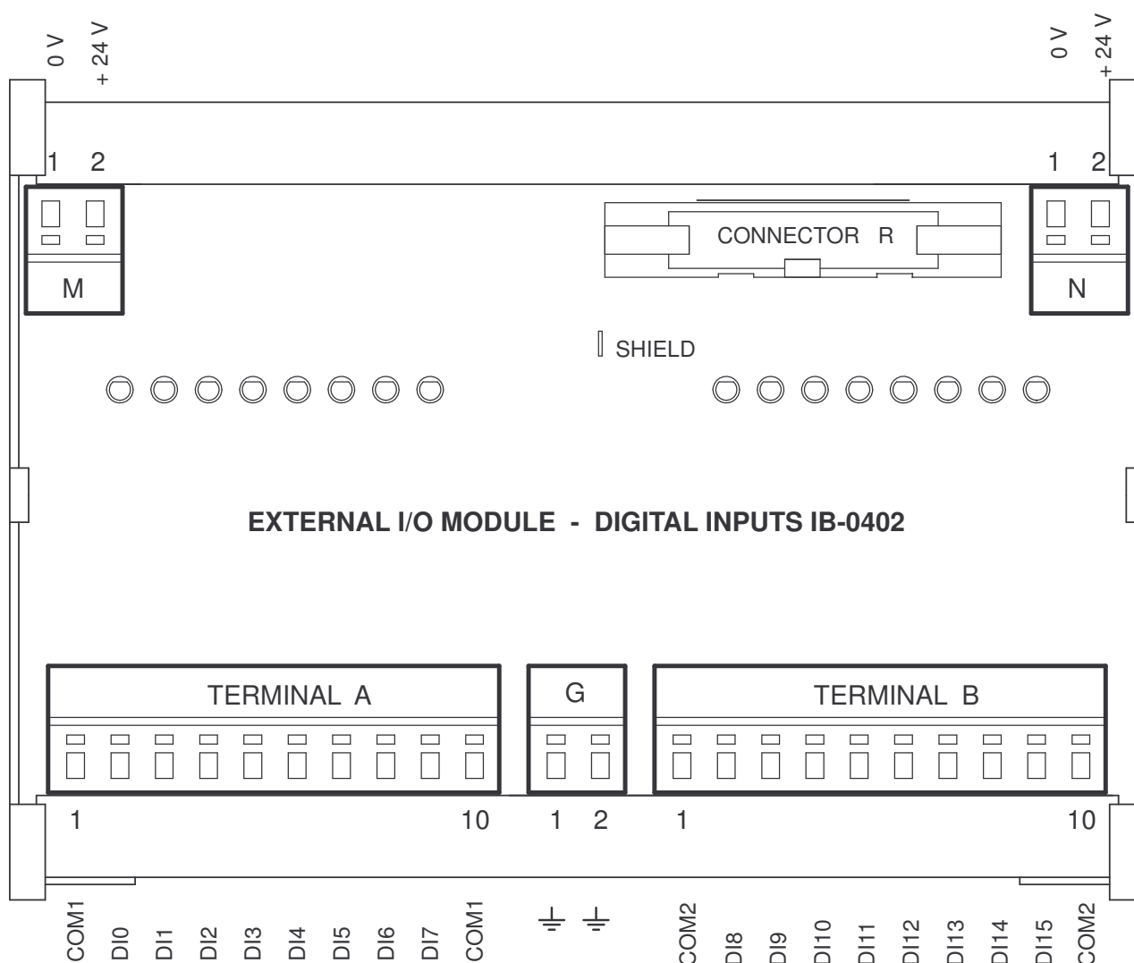
Fig. 5.1: Connection of connector of the IB-0402 module
