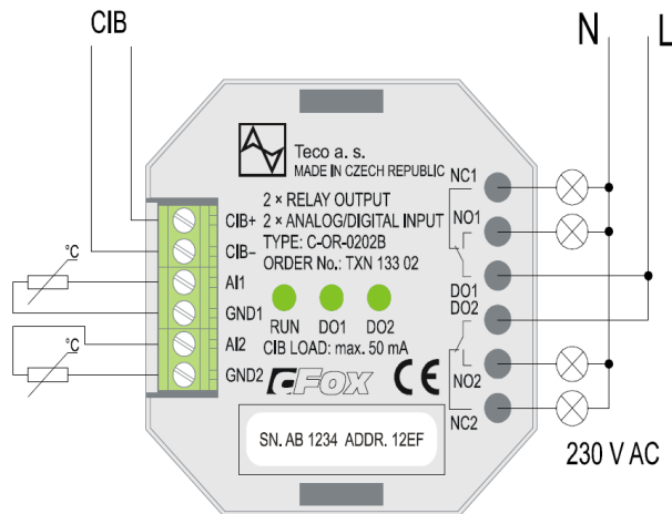
Fig. 3. 62 view C-OR-0202B
