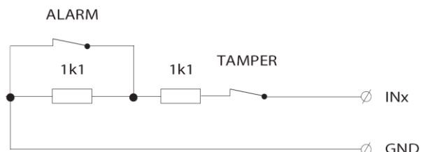
Fig. 3. 55 Double-balanced input for security detectors
