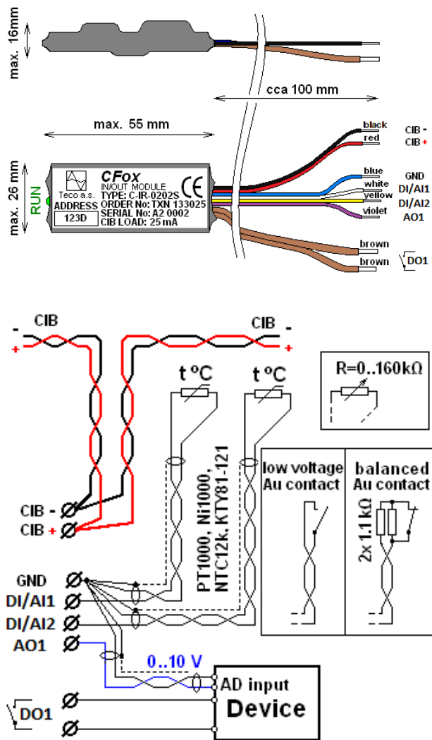
Fig. 3.19 View and connection C-IR-0202S
