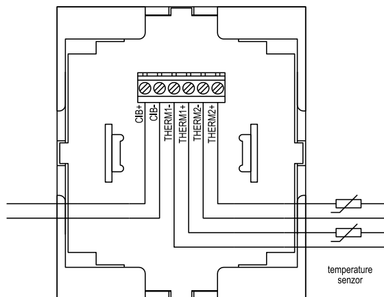
Fig. 3. 82 View and connection example
