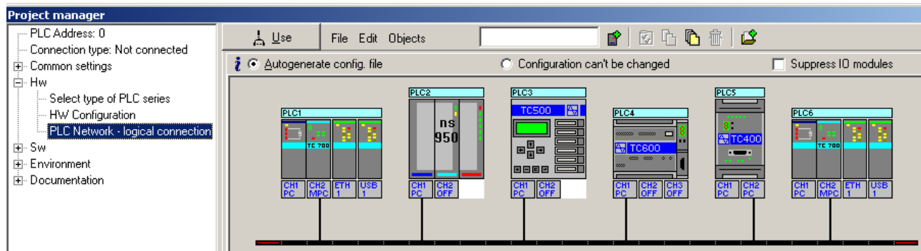
Fig.2.4.2 PLC network creation according to an example
