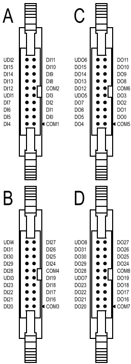
4× 20pin DIN 41651 Flat Cable Connector
